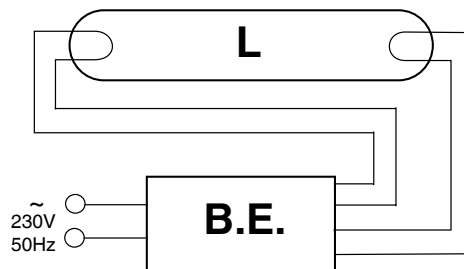
Schita montaj balast electronic:
