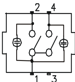
Schema electrica
