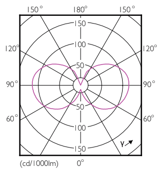
LED Bulb CLA 8-50W E27 G120 Amber 822 DIM
