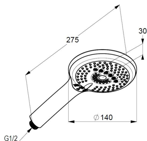
Dimensional drawing
