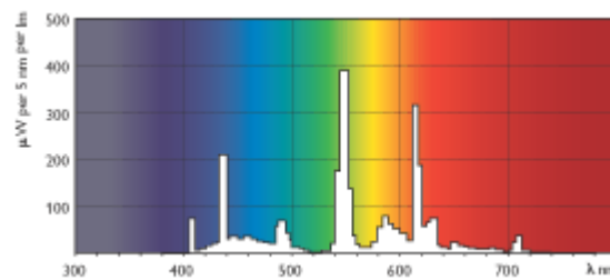
Lightcolor /840 MASTER PL-C/840
