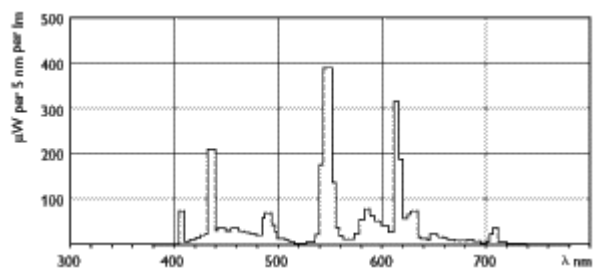
Lightcolor /840 MASTER PL-C/840
