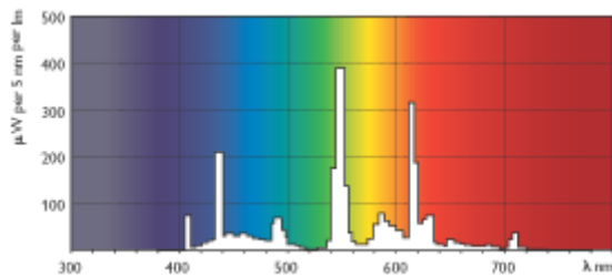
Lightcolor /840 MASTER PL-L/840
