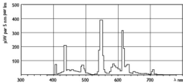
Lightcolor /840 MASTER PL-L/840
